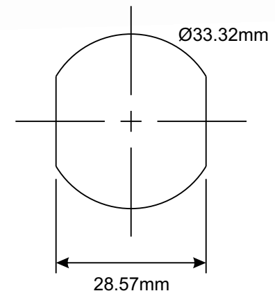
Panel Cutout
