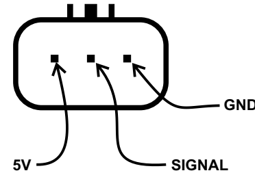
Pin Allocations
