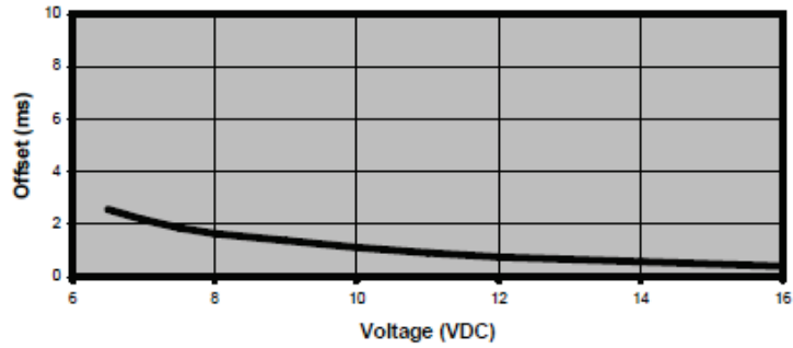
Voltage Sensitivity Summary, 6-16V
