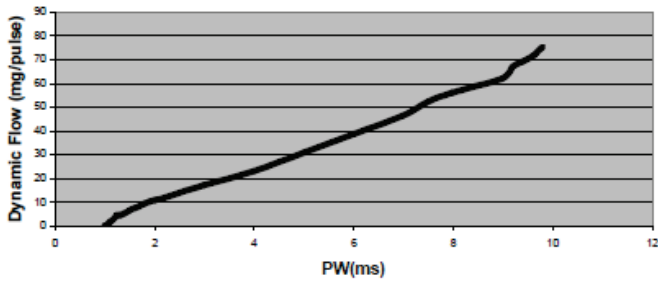
Characteristic Injector Flow Curve
